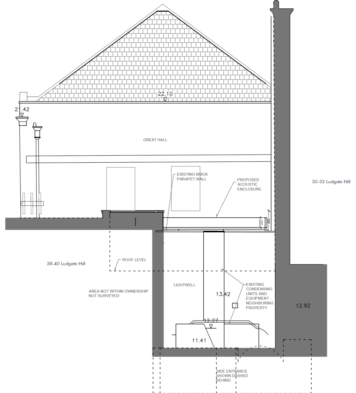
Existing & proposed section CC
