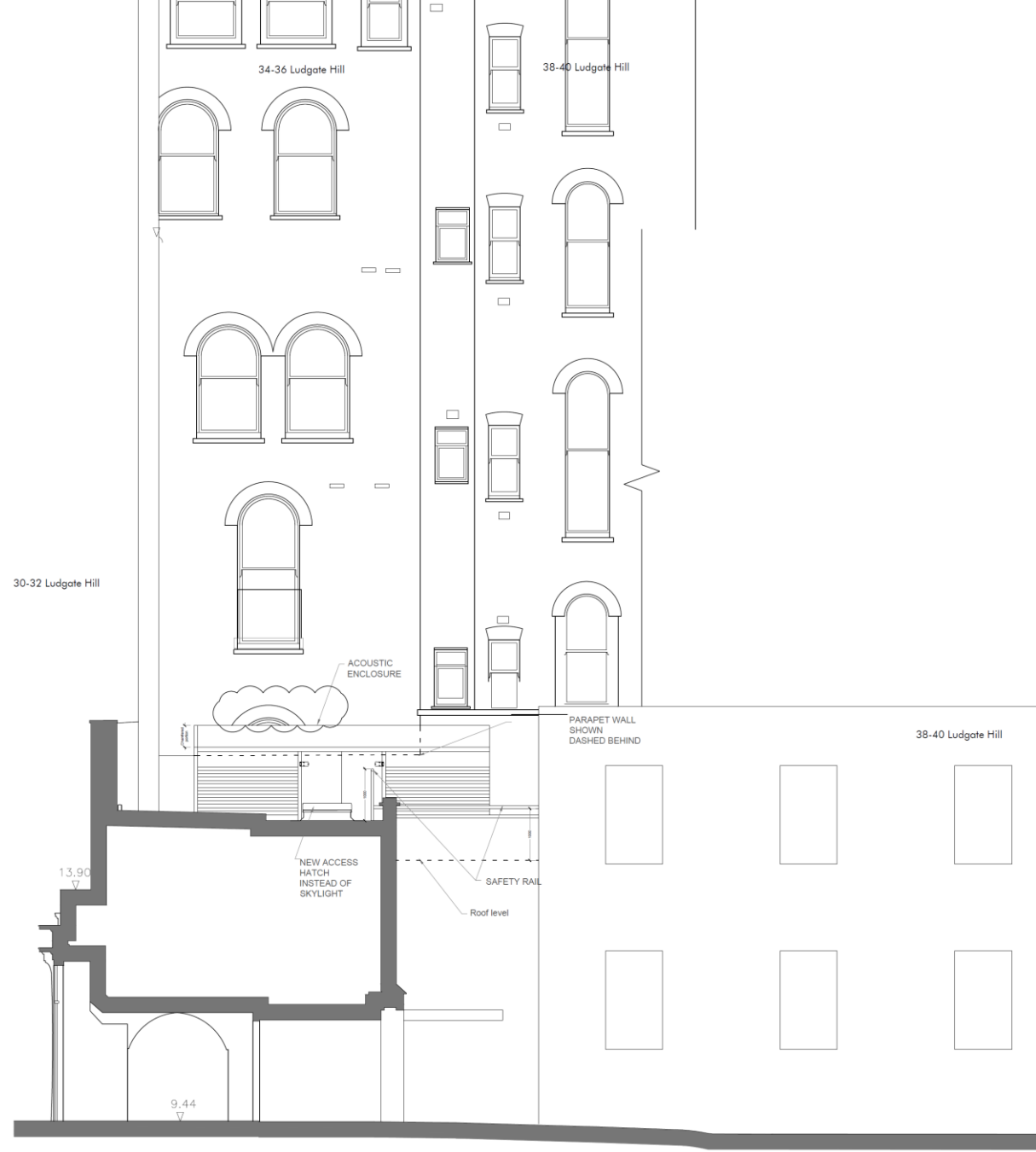
Proposed section DD & EE
