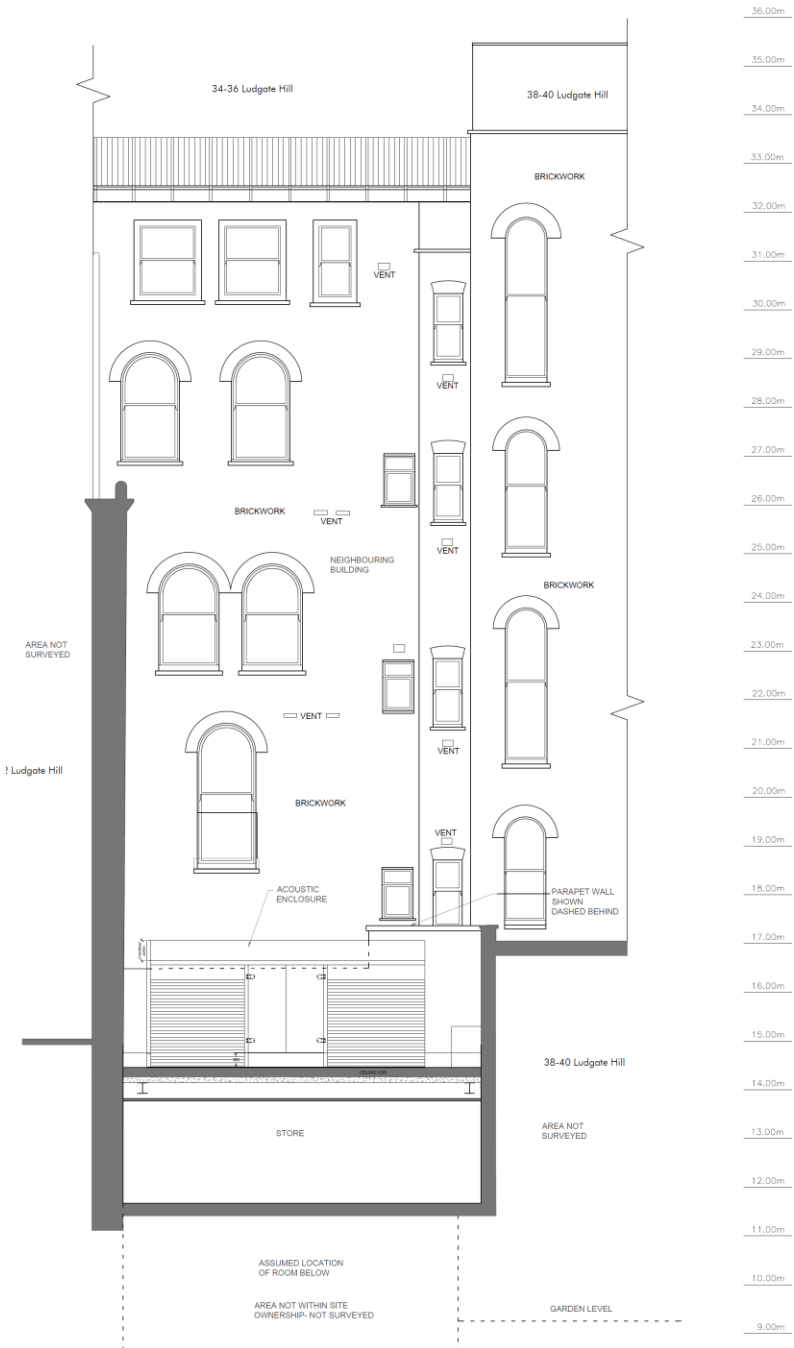
Existing & proposed section BB
